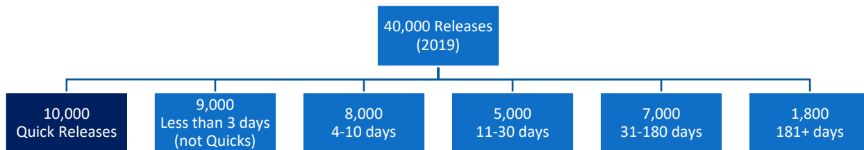
Figure 32: Release Timing, 2019
